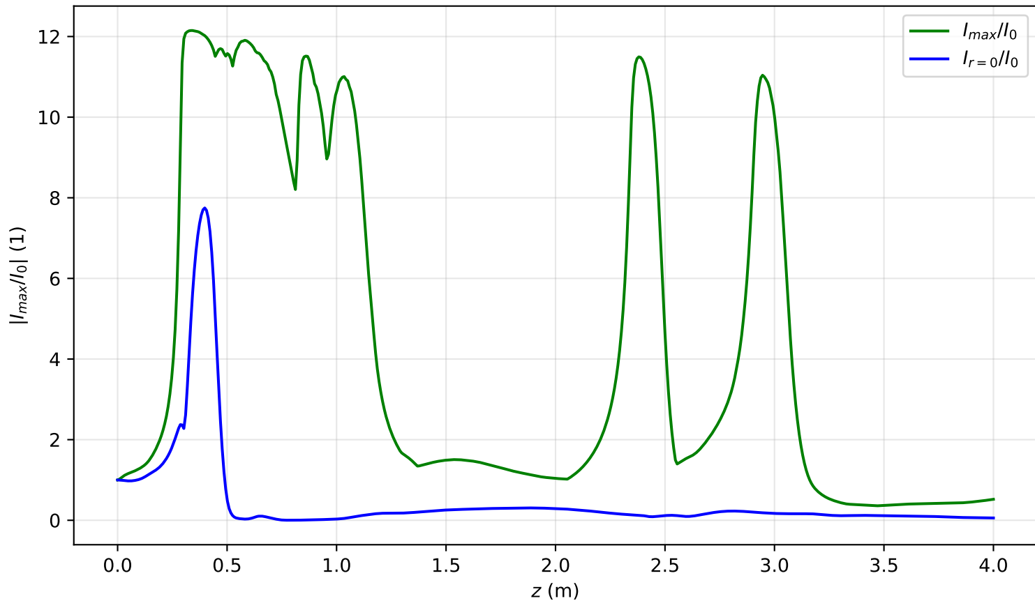
I_{max}(x = 0, y = 0, z)/I_0 , P_{in}=9.1P_{cr} , noisy input, artificial time
